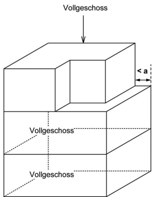
Figur 6.4 Attikageschosse
