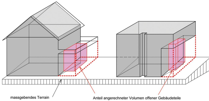
Figur 8.3 Baumassenziffer
